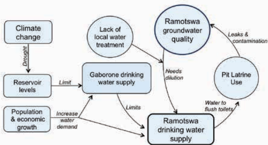
FIGURE 6. Conceptual diagram of the connections between climate, water and sanitation infrastructure, and groundwater quality in Ramotswa, Botswana.
