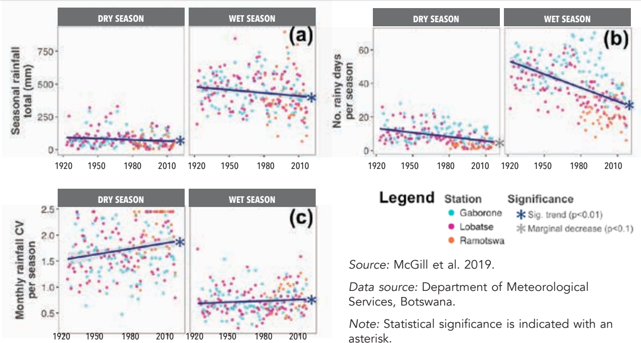
FIGURE 5. Dry- and wet-season rainfall patterns over time at Gaborone, Lobatse and Ramotswa weather stations. (a) total rainfall, (b) number of rainy days, and (c) seasonal coefficient of variation (CV) among monthly rainfall totals, i.e., seasonal rainfall variability.
